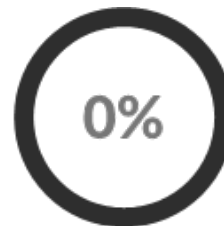
Load balancing
